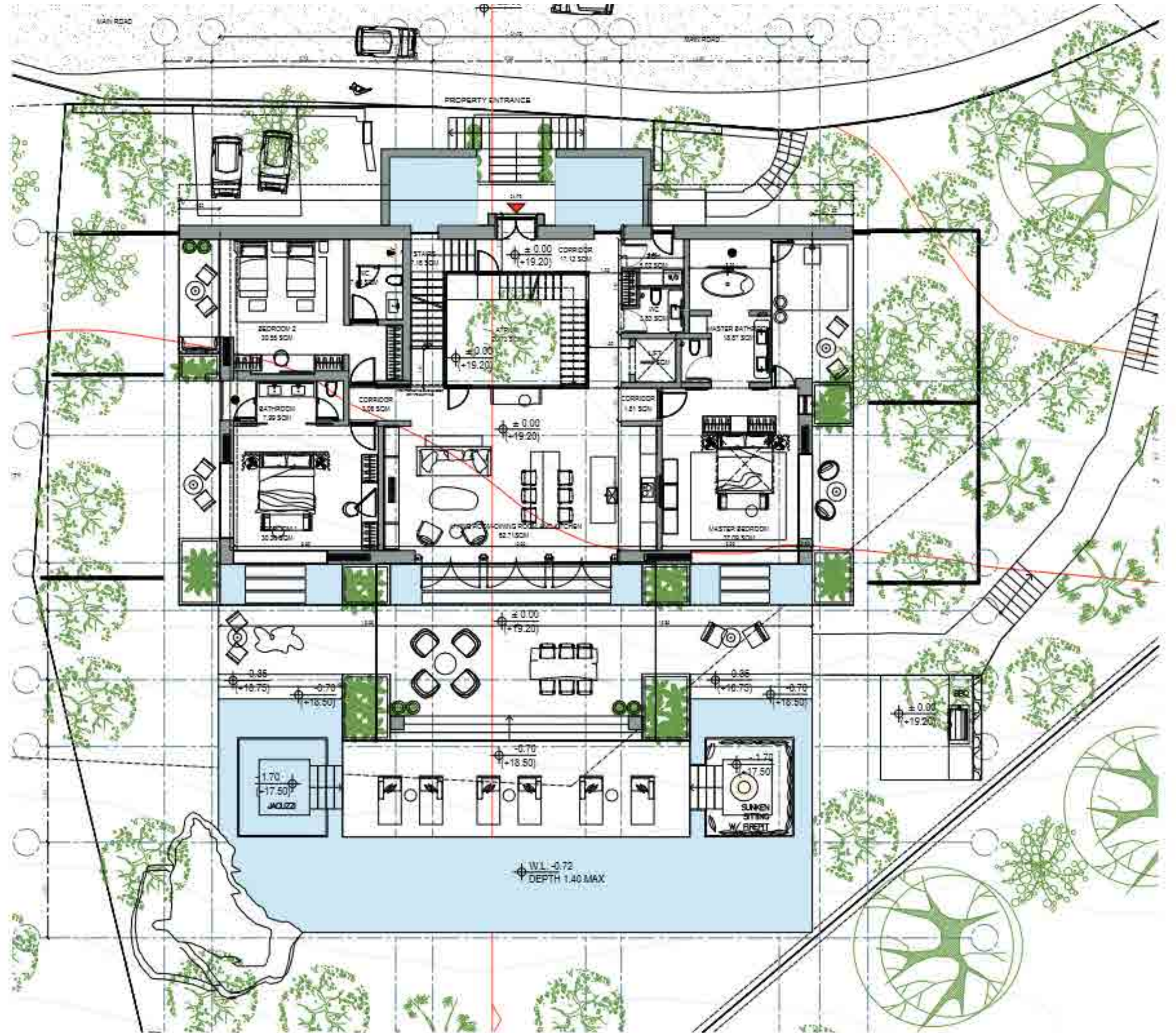
FREEHOLD VILLA – 260 SQM – GROUND FLOOR
