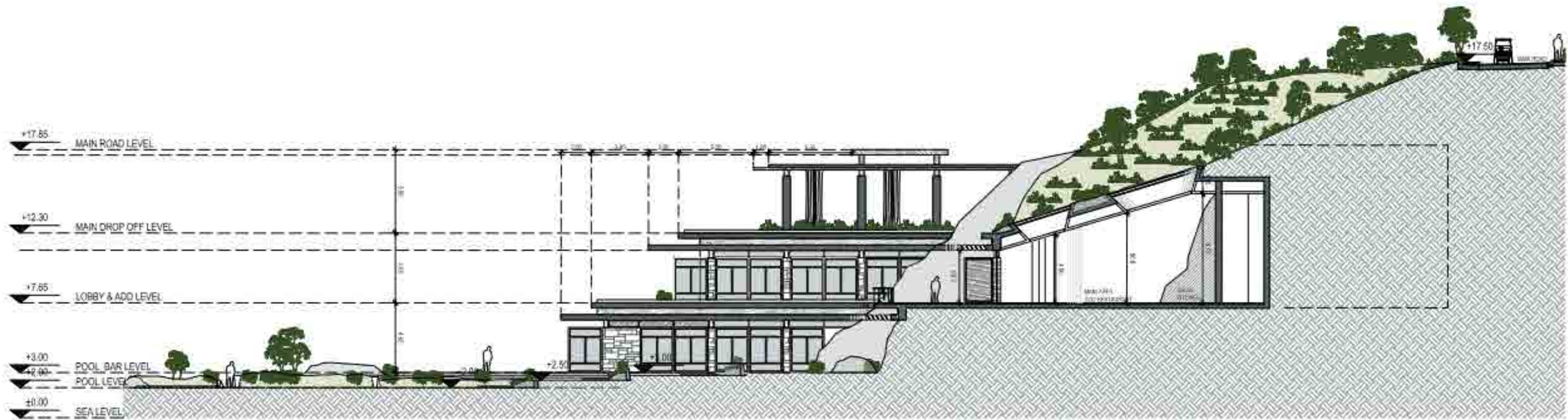
SECTION B-B
