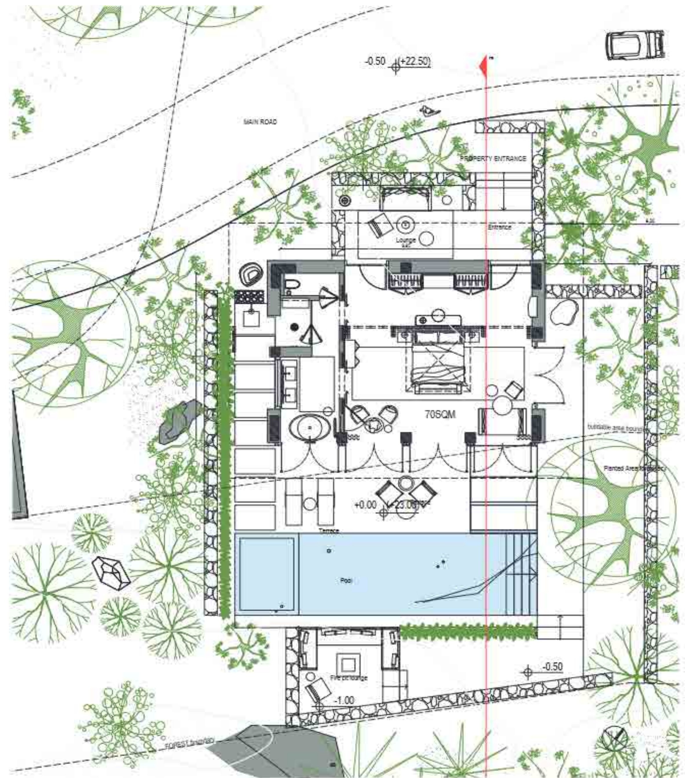
HOTEL VILLA 70 – GROUND FLOOR PLAN
